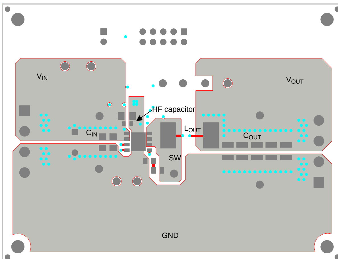
Figure 41. Top Layer
