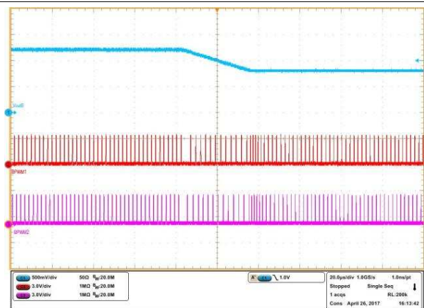
V_{IN} = 1.2\text{ V} I_{OUT\_B} = 30\text{ A} V_{OUT\_B} VID step from 1.2 V to 0.8 V
