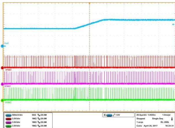
V_{IN} = 12\text{ V} I_{OUT\_A} = 30\text{ A} V_{OUT\_A} VID step from 0.8 V to 1.2 V
