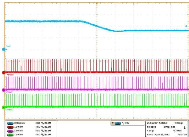
V_{IN} = 12\text{ V} I_{OUT\_A} = 30\text{ A} V_{OUT\_A} VID step from 1.2 V to 0.8 V
