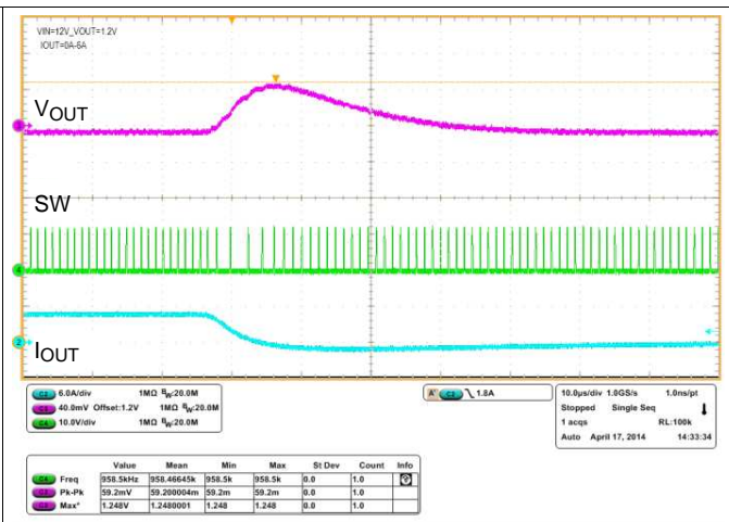
I_{LOAD} from 6A to 0 A
