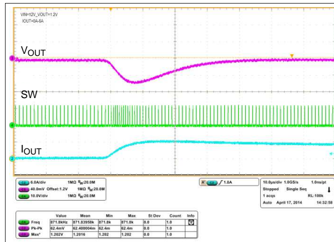
I_{\text{LOAD}} from 0 A to 6 A
