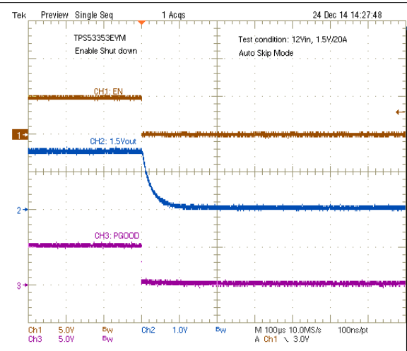
Figure 8-3. Enable Turnoff
