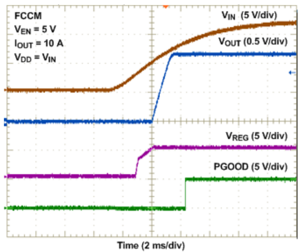
Figure 9-16. UVLO Start-Up
