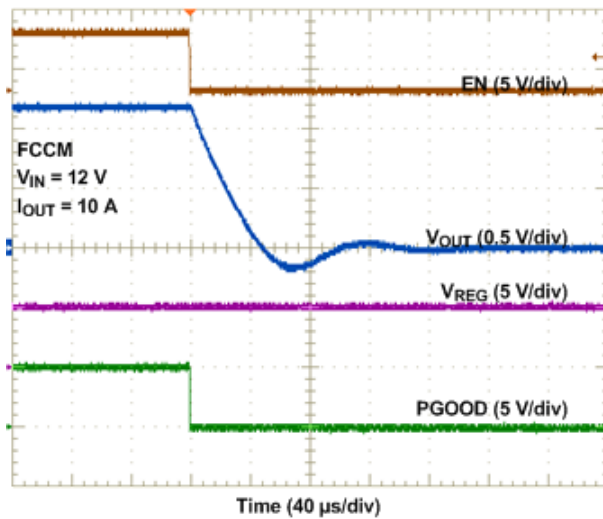
Figure 9-15. Shutdown
