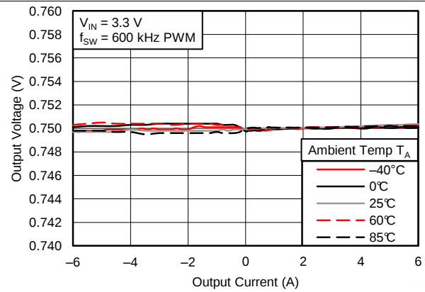
Figure 12. Load Regulation
