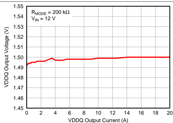
Figure 16. Load Regulation
