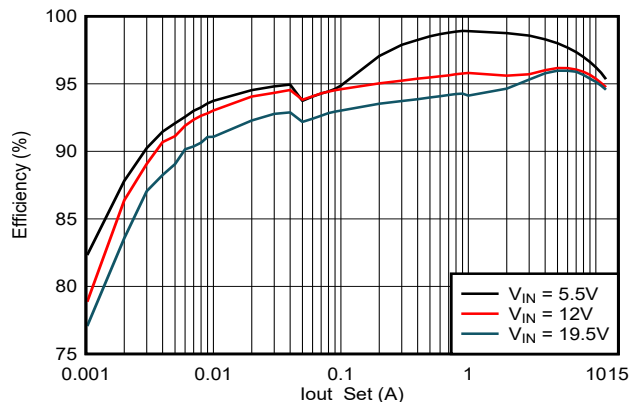
Efficiency vs Output Current, 560kHz, Eco-mode
