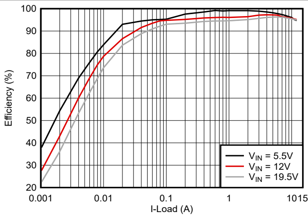
Figure 5-15. Efficiency vs Load Current, 560kHz, OOA Mode
