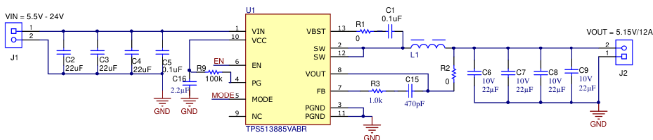
Figure 7-1. 5.15V, 12A Reference Design
