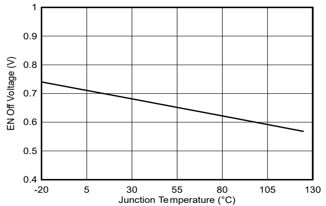
Figure 5-4. Enable Off Voltage vs Junction Temperature
