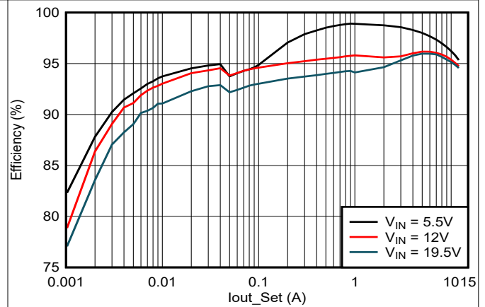
Figure 5-16. Efficiency vs Load Current, 560kHz, Eco-mode
