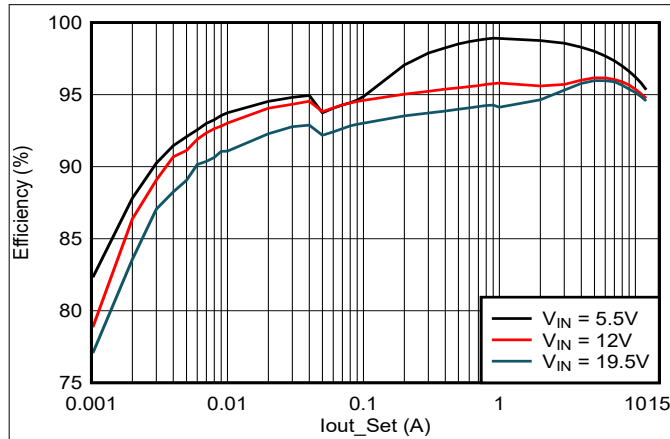
Figure 7-2. Efficiency Curve (ECO)
