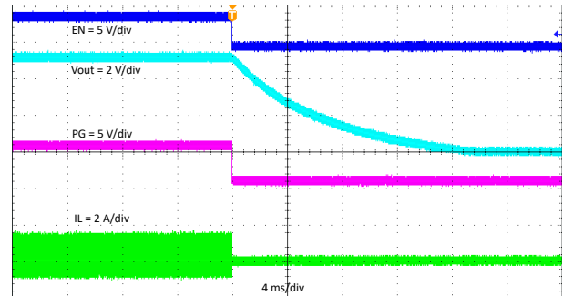
Figure 8-9. Shutdown Relative to EN Falling, Iout = 0.01 A, OOA Mode
