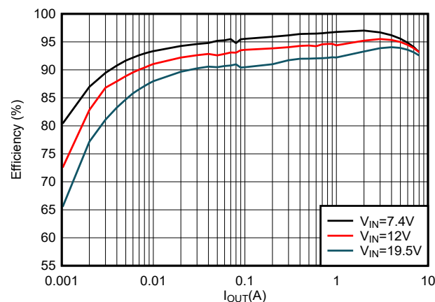
Efficiency Curve, V_{OUT} = 5.1\text{ V} , PSM Mode
