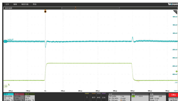
Figure 8-15. Transient Response, 1.4 A to 5.6 A with 2.5 A/us SR
