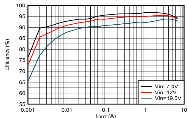
Efficiency Curve, V_{OUT} = 5.1 V, PSM Mode
