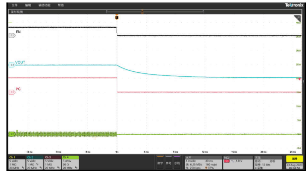
Figure 8-9. Shutdown Relative to EN Falling, Iout = 0A, OOA Mode
