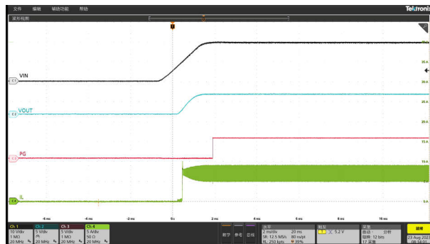
Figure 8-10. Start-Up Relative to Vin Rising, Iout = 7A
