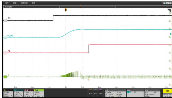
Figure 8-8. Start-Up Relative to EN Rising, Iout = 0A, OOA Mode
