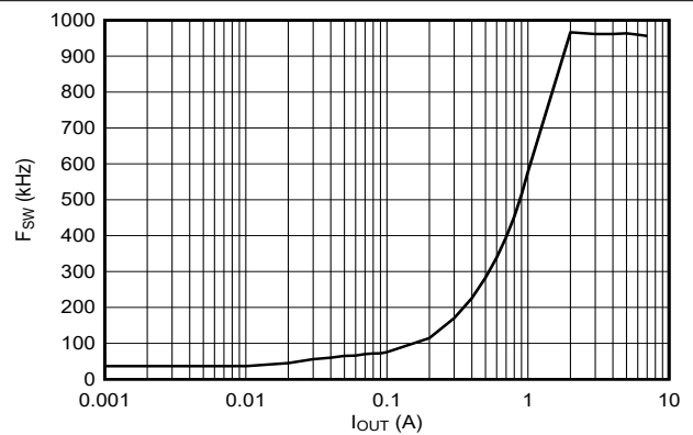
Figure 8-5. Switching Frequency, OOA Mode
