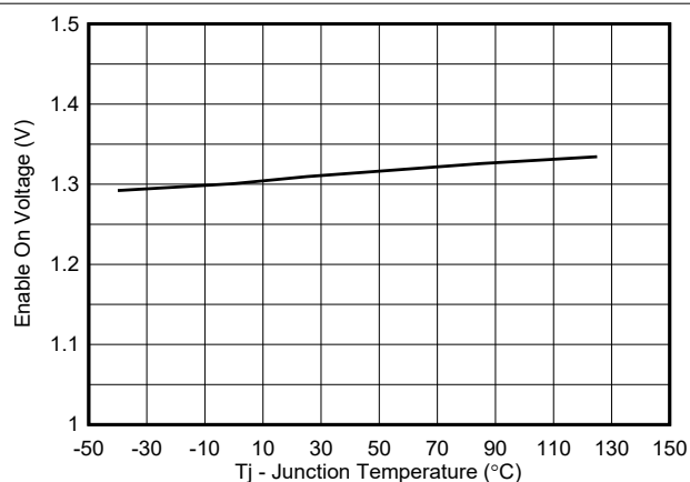
Figure 6-4. Enable On Voltage vs Temperature
