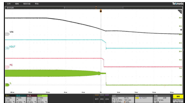
Figure 8-11. Shutdown Relative to Vin Falling, Iout = 7A
