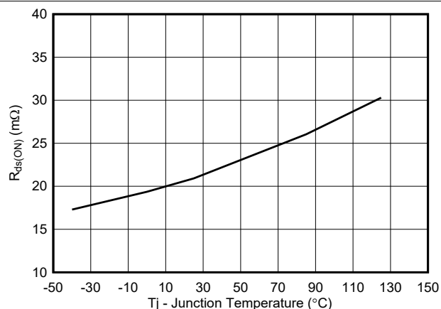
Figure 6-6. High-side R_{DS(on)} vs Temperature
