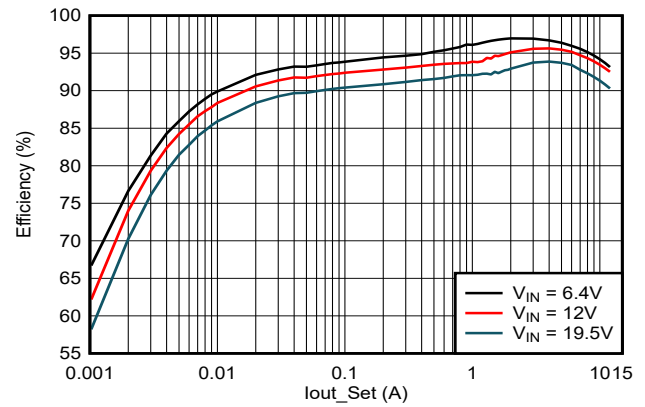
Figure 7-4. Efficiency Curve ( V_{OUT} = 3.3V )
