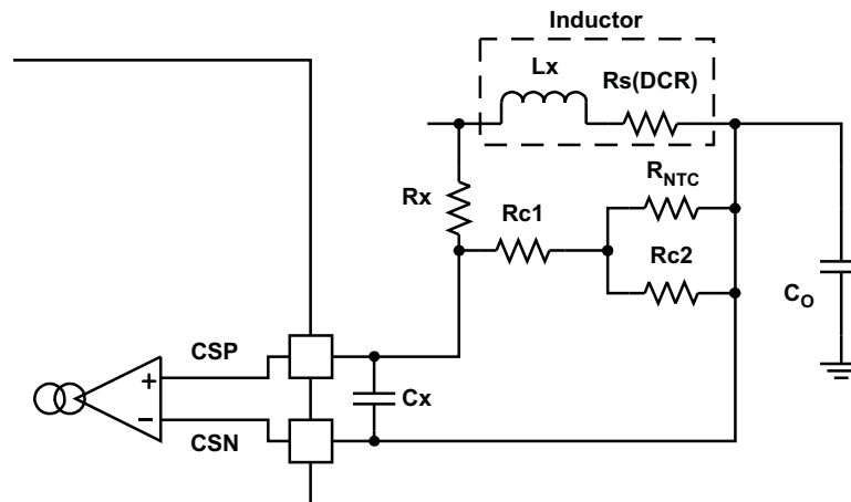
Figure 50. Inductor DCR Current Sensing With Temperature Compensation
