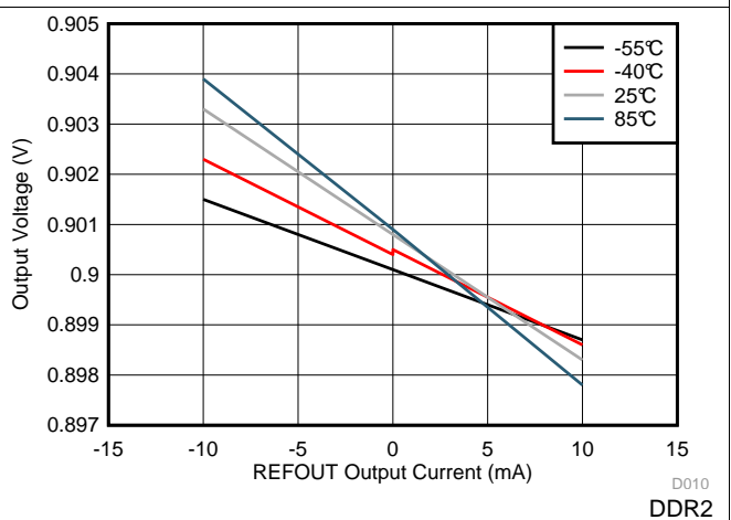
Figure 11. REFOUT Load Regulation
