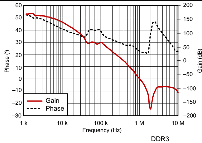
Figure 16. Bode Plot
