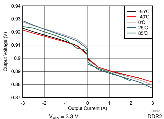
Figure 3. Load Regulation
