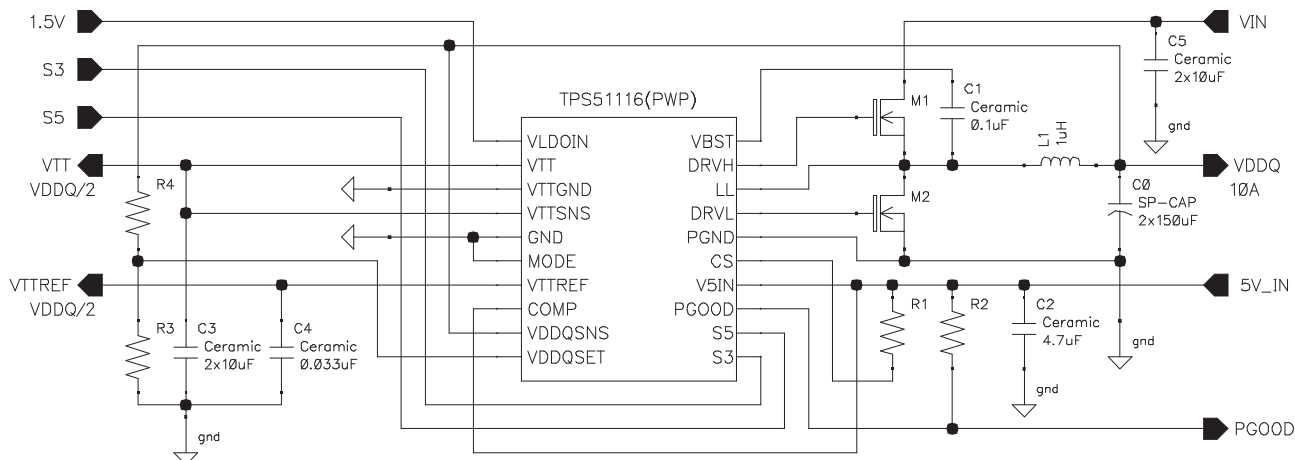
Figure 6. D-CAP™ Mode
