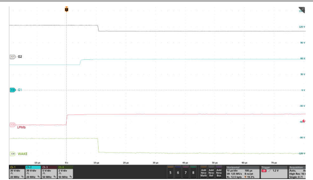
Figure 8-5. State Transition From LPM to Active Mode ( \overline{\text{LPM}} = \text{Low to High} , V_{\text{IN}} = 48\text{V} , No Load)
