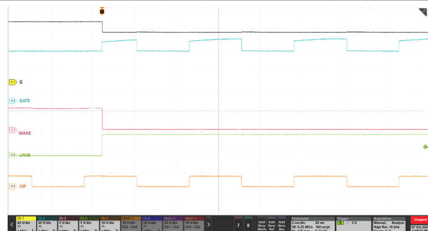
Figure 9-7. With \overline{\text{LPM}} = Low to High, \text{INP} Gained Control on GATE ( V_{\text{IN}} = 48V, No Load)
