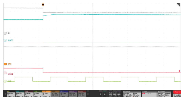
Figure 9-5. When \overline{\text{LPM}} = Low in LOAD WAKEUP state, \text{INP} Has No Control on GATE
