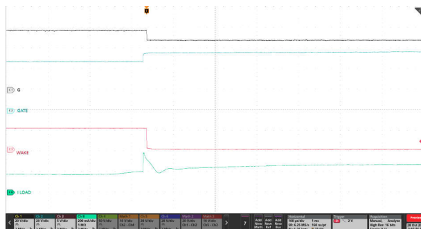
Figure 9-4. Zoom-In View of State Transition From LPM to Active Mode ( \overline{\text{LPM}} = Low, V_{\text{IN}} = 48V, \text{EN}/\overline{\text{UVLO}} = High)
