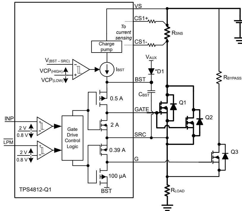
Figure 8-1. Gate Driver
