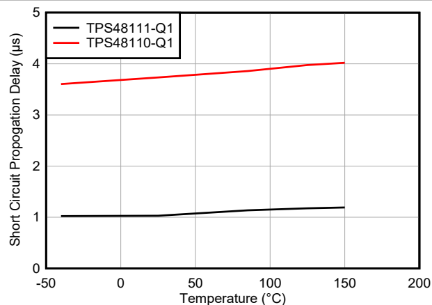
Figure 6-12. Short-Circuit Protection Response Time ( t_{sc} ) vs Temperature
