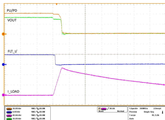
Figure 9-13. Output Hot-Short Response of the TPS48110-Q1 Device
