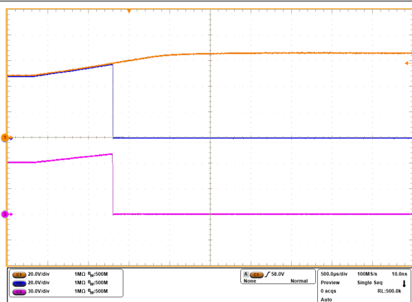
Figure 8-10. Overvoltage Cutoff Response of TPS4800-Q1 at 58V Level
