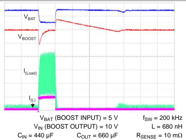
Figure 9. Load Step Response (Boost) (0 to 5 A at 10 A/ \mu s)
