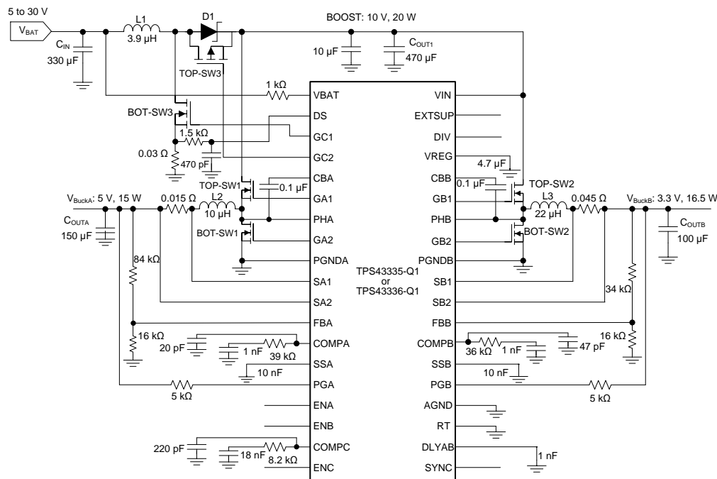
Figure 32. Simplified Automotive ADAS Supply Schematic
