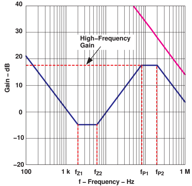
Figure 25. Type-III Compensation Network Typical Bode Plot
