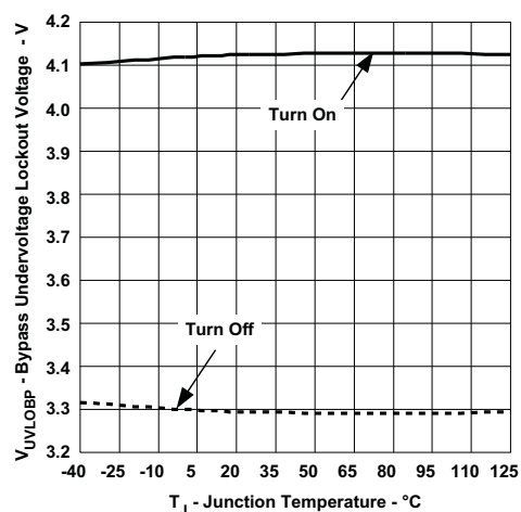
Figure 12. BP Undervoltage Lockout Voltage vs Junction Temperature
