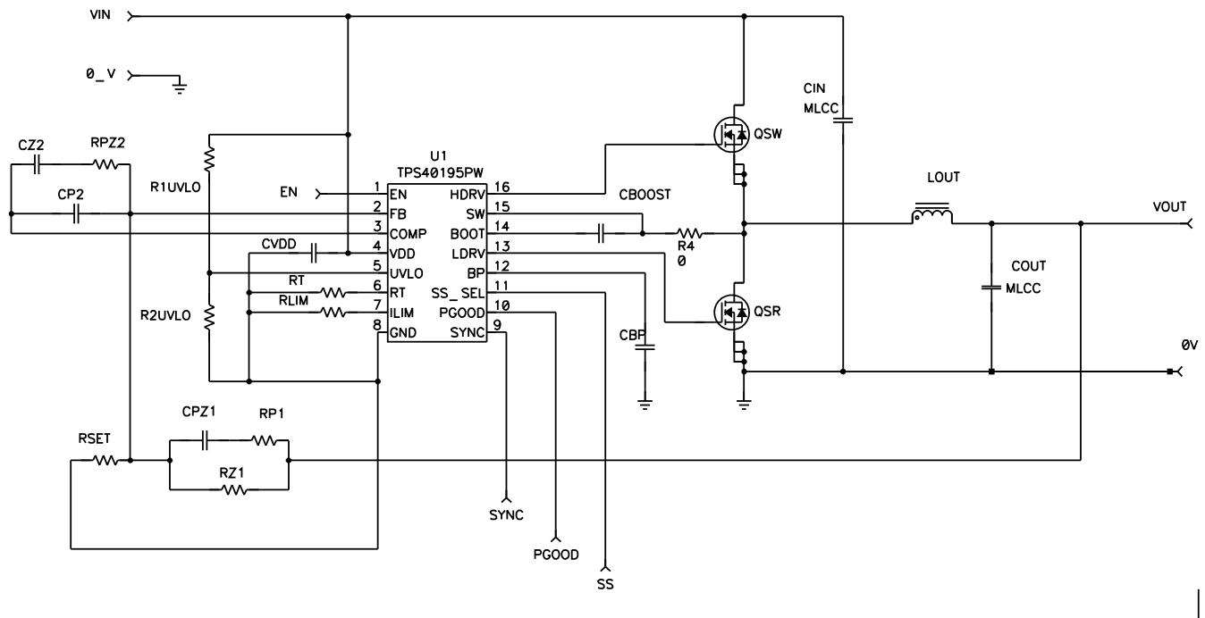
Figure 22. TPS40195 Design Example Schematic
