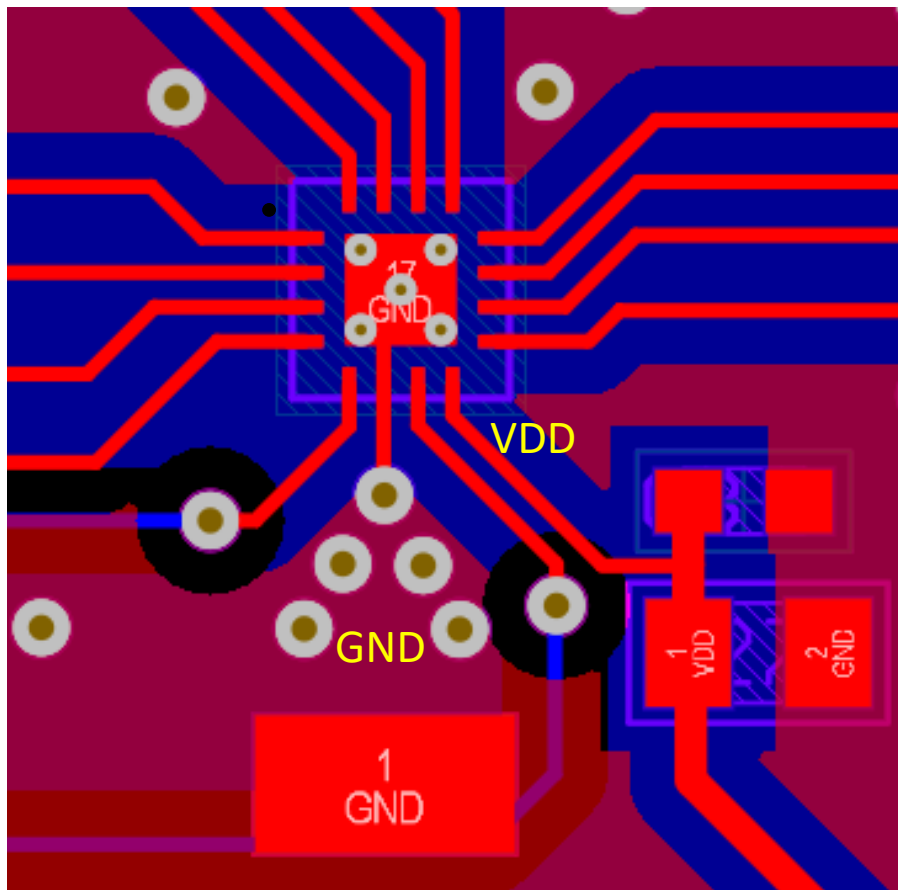
Figure 9-13. Recommended Layout
