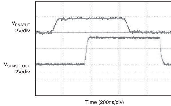
Figure 17. Enable Power On and Power Off Delay (TPS3895P)
