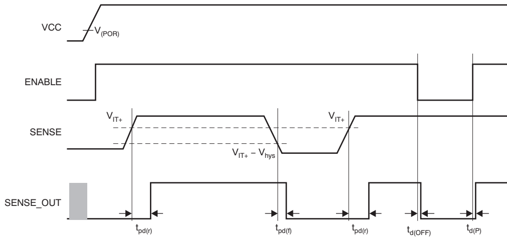
Figure 2. TPS3895P and TPS3897P Timing
