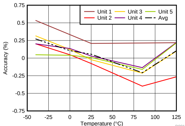
V_{ITN} Accuracy vs Temperature
