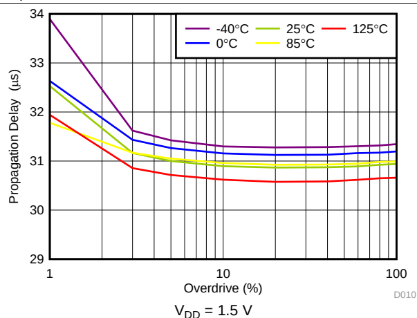
Figure 14. Propagation Delay ( t_{\text{PD}(f)} ) vs Overdrive
