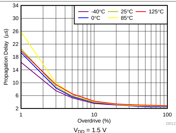
Figure 16. Propagation Delay ( t_{\text{PD}(f)} ) vs Overdrive
