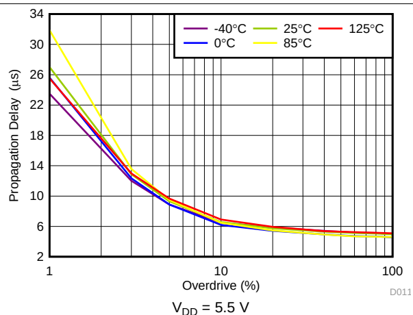
Figure 15. Propagation Delay ( t_{\text{PD}(f)} ) vs Overdrive
