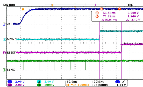
Figure 9-7. Power Up Sequence with SYNC
