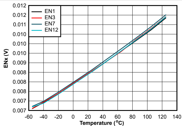
Figure 7-6. ENx Logic Low Output Voltage vs. Temperature
