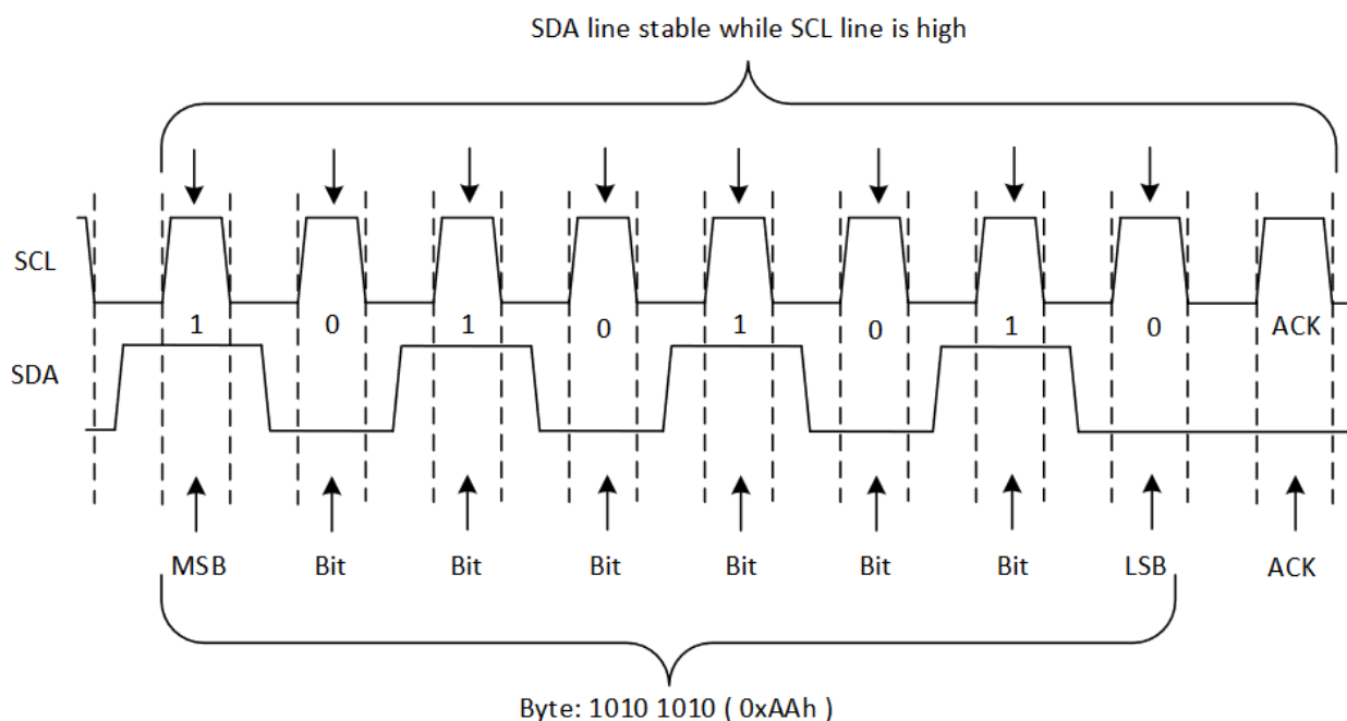
Figure 8-7. SCL to SDA Timing for 1 Byte Data Transfer
