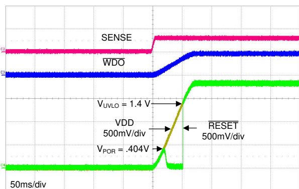
Figure 8-7. Startup Waveform
