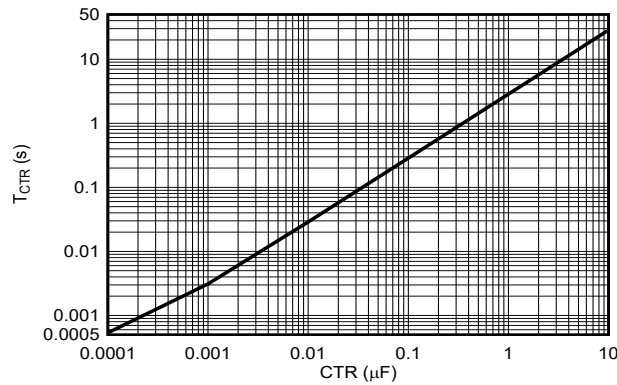
Figure 6-4. T_{\text{CTR}} vs \text{CTR}
