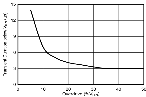
Figure 6-6. Transient Duration at Sense vs Sense Threshold Overdrive Voltage ( \text{CTS} = \text{Open} )
