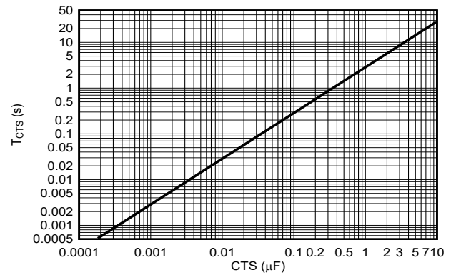
Figure 6-5. T_{\text{CTS}} vs \text{CTS}
