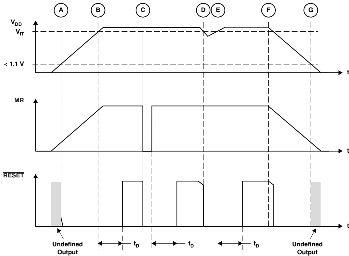
Figure 7. Timing Diagram
