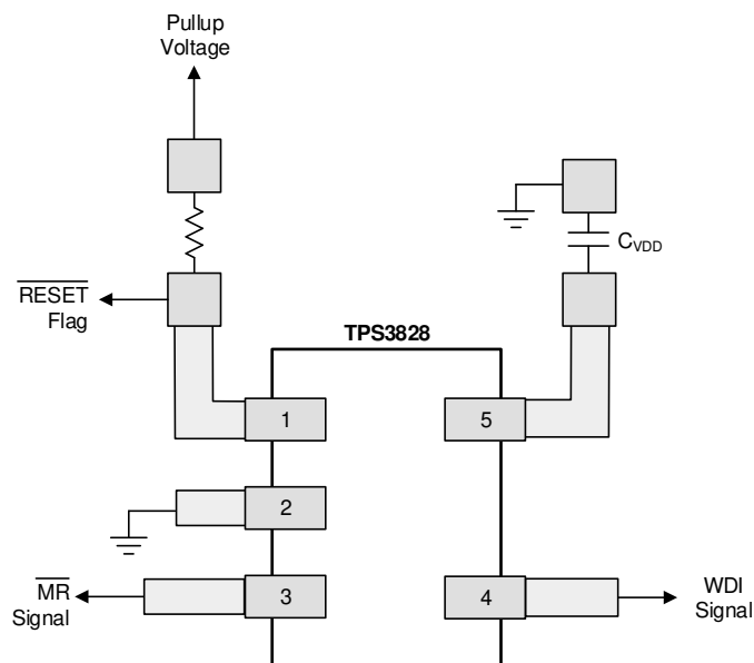
Figure 8-5. Example Layout (DBV Package)
