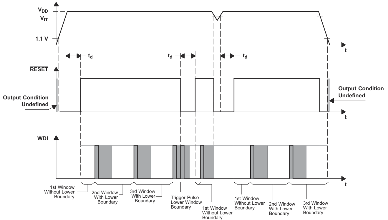
Figure 6-1. Timing Diagram
