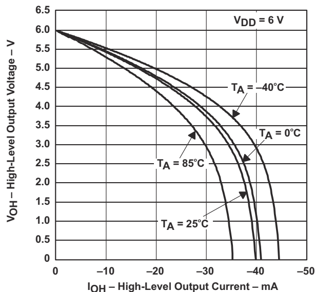
Figure 7-3. HIGH-LEVEL OUTPUT VOLTAGE vs HIGH-LEVEL OUTPUT CURRENT at V_{DD}=6V
