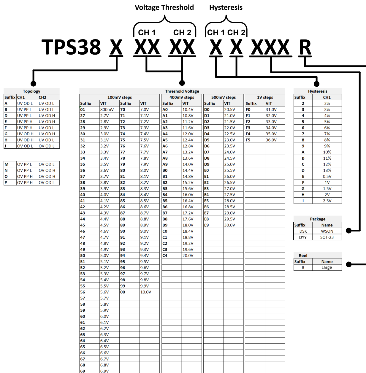
Figure 5-1. Device Nomenclature
