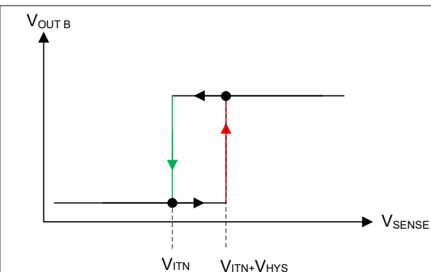
Figure 7-5. Hysteresis (Undervoltage Active-Low)
