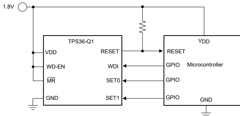
Figure 9-1. Monitoring Microcontroller Supply and Watchdog During Operation and Sleep
