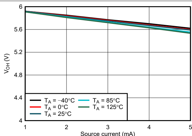
Figure 7-17. WDO V_{OH} vs I_{source} , V_{DD} = 6.0\text{ V}
