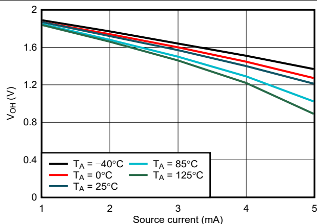
Figure 7-15. WDO V_{OH} vs I_{source} , V_{DD} = 2.0\text{ V}
