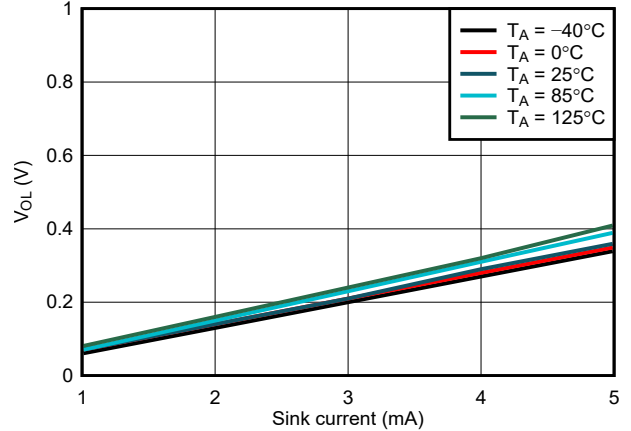
Figure 6-11. WDO V_{OL} vs I_{sink} , V_{DD} = 1.5V
