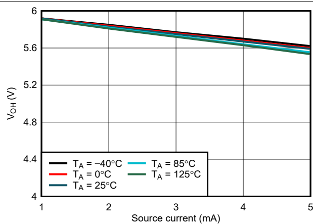
Figure 6-9. WDO V_{OH} vs I_{source} , V_{DD} = 6.0\text{V}
