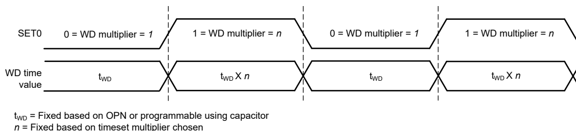
Figure 7-11. Watchdog Operation with 1 SET Pin
