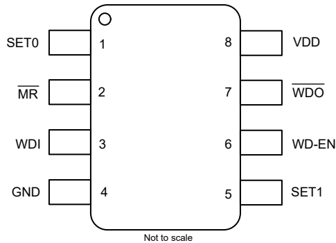
Figure 5-3. Pin Configuration Option C DDF Package, 8-Pin SOT-23, TPS3435 Top View
