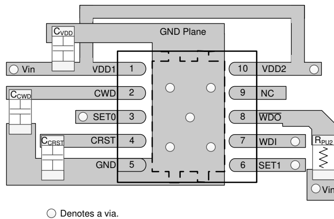
Figure 10-1. Typical Layout for the TPS3430-Q1
