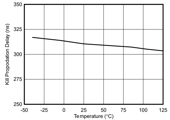
Figure 6-12. Kill Propagation Delay vs Temperature
