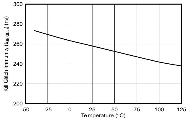
Figure 6-13. Kill Glitch Immunity vs Temperature
