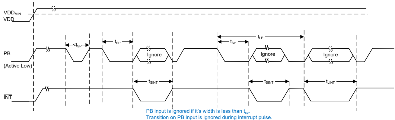
Figure 7-5. Push Button Functionality
