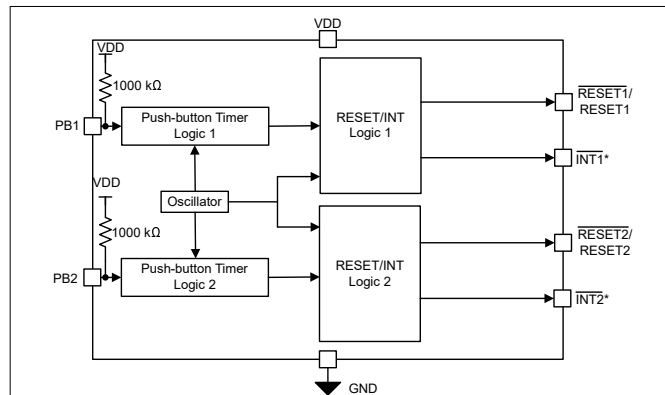
Figure 7-1. TPS3423 Block Diagram (Active Low Push-Button Input)
