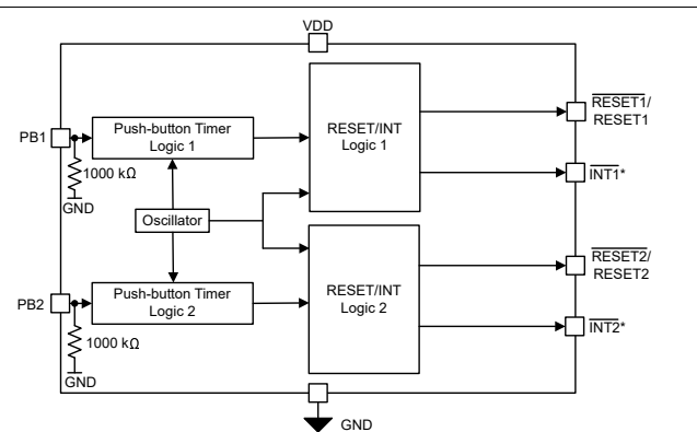
Figure 7-2. TPS3423 Block Diagram (Active High Push-Button Input)
