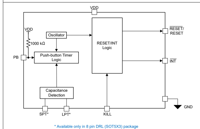
Figure 7-3. TPS3424 Block Diagram (Active Low Push-Button Input)
