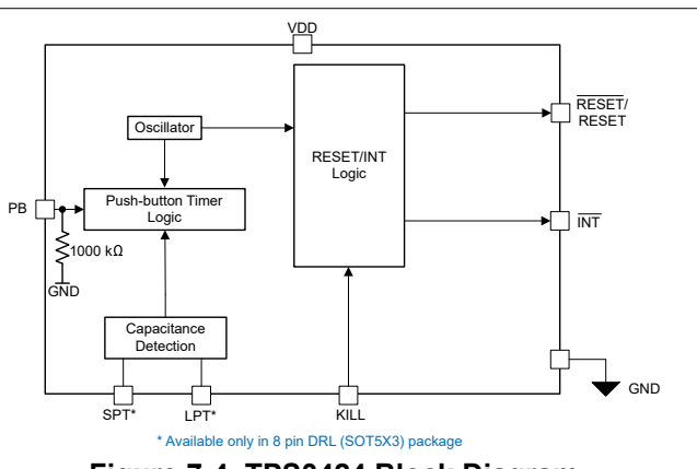
Figure 7-4. TPS3424 Block Diagram (Active High Push-Button Input)
