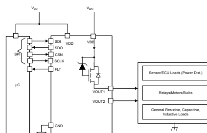
Simplified Schematic
