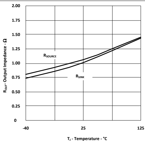
V_{DD} = 7.2 \text{ V} Figure 5-6. UGATE DC Output Impedance vs Temperature
