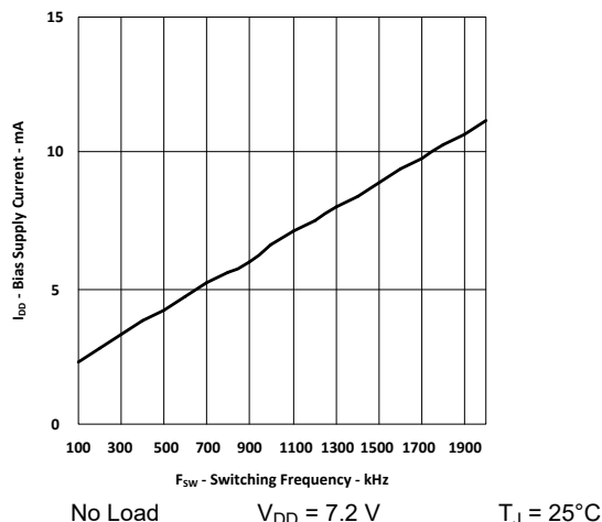
Figure 5-14. Bias Supply Current vs Switching Frequency
