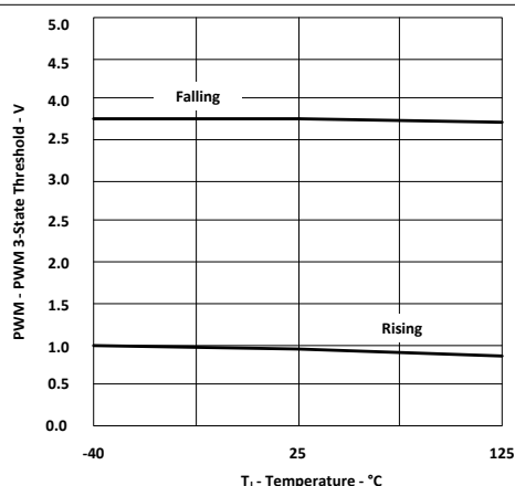
V_{DD} = 7.2 \text{ V} Figure 5-5. PWM 3-State Thresholds, (5-V Input Pulses) vs Temperature
