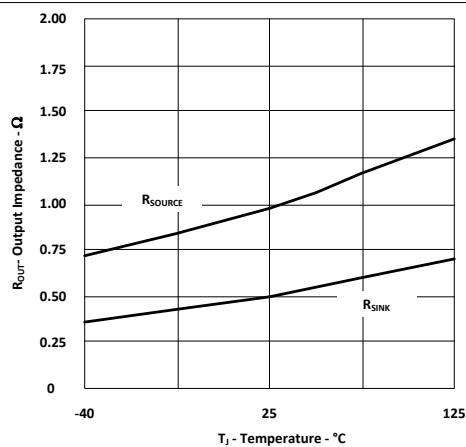
V_{DD} = 7.2 \text{ V} Figure 5-7. LGATE DC Output Impedance vs Temperature
