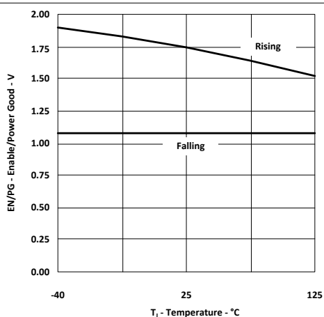
V_{DD} = 7.2 \text{ V} Figure 5-4. Enable/Power Good Threshold vs Temperature
