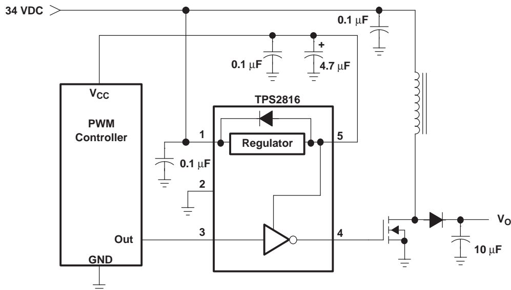
Figure 22. Boost Application
