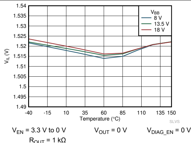
Figure 7-22. V_{IL} vs Temperature
