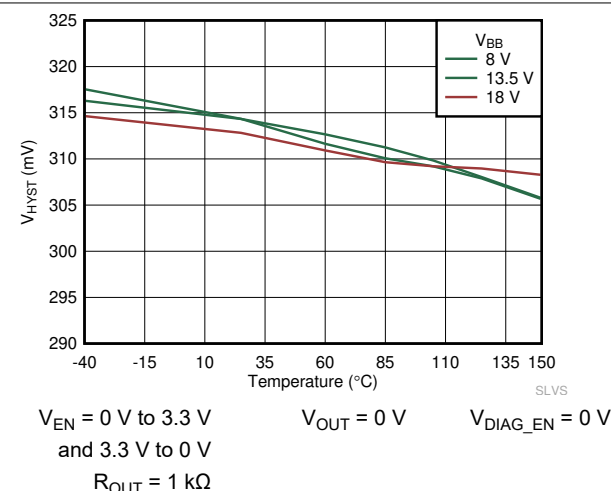
Figure 7-24. V_{IHYS} vs Temperature
