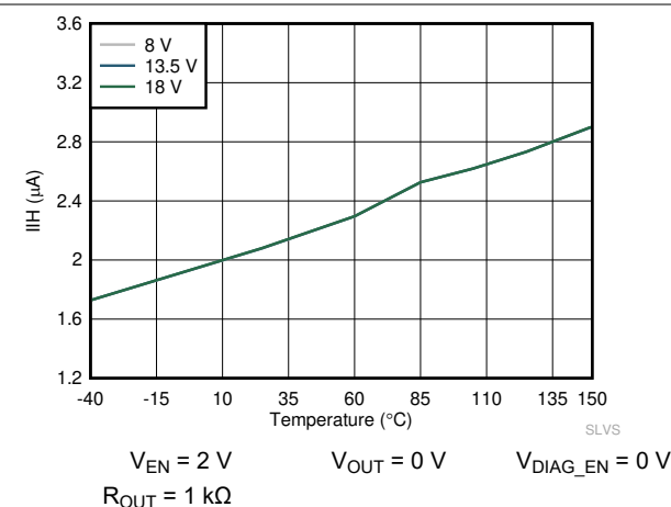
Figure 7-26. I_{IH} vs Temperature
