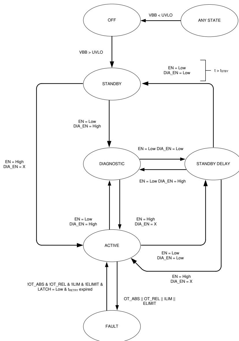
Figure 9-11. State Diagram
