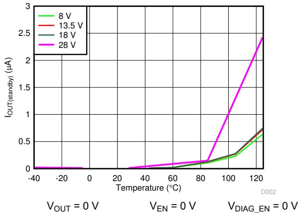
Figure 7-3. Output Leakage Current ( I_{OUT(standby)} ) vs Temperature
