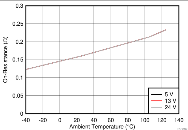
Figure 7-12. Channel-3 FET On-Resistance
