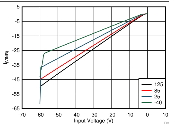
Figure 7-10. Input Supply Current vs Reverse Supply Voltage, -V_{(IN)}
