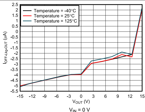
Figure 7-11. I OFF-Leakage-OUT vs V OUT
