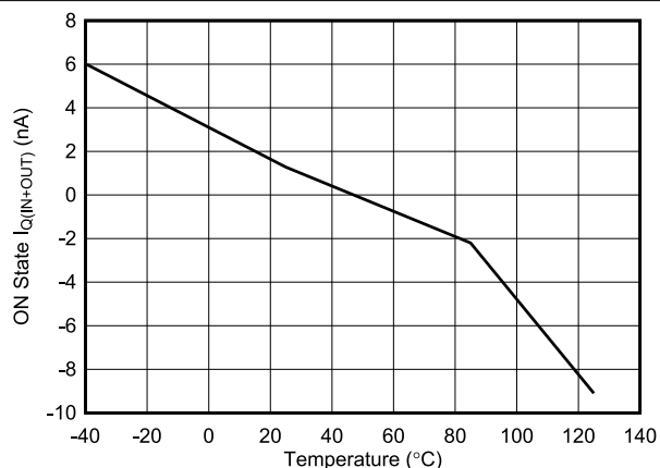
Figure 7-2. I_Q \text{ (IN+OUT)} vs Temperature in Normal Operation
