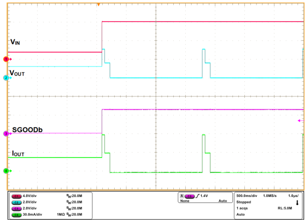
Figure 8-9. Auto-Retry Behavior
