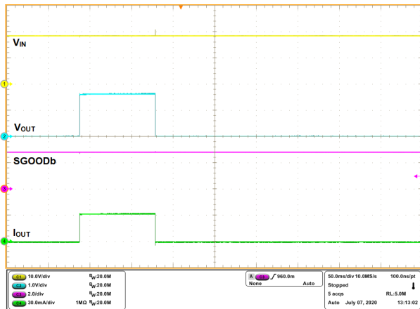
Figure 9-2. Current Limiting with MODE = GND, R_{burden} = 50\ \Omega
