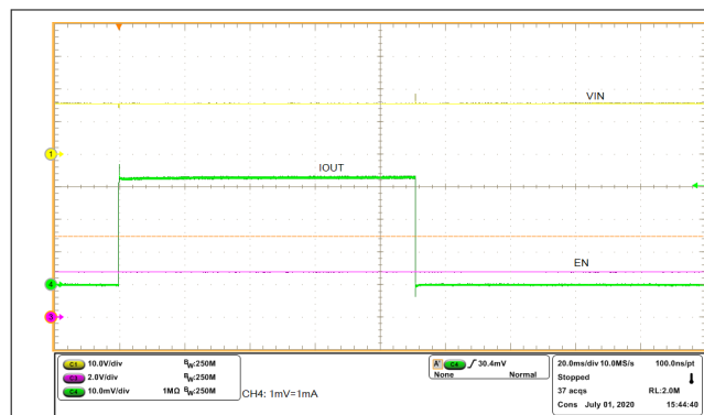
Figure 8-6. Current Limit Behavior for I_{OUT} < 2 \times I_{OL} with MODE = GND
