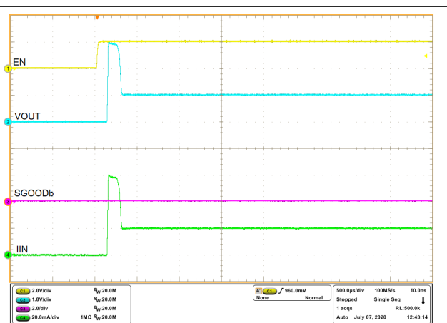
Figure 9-10. Enable Control with TPS26611 (EN = High)
