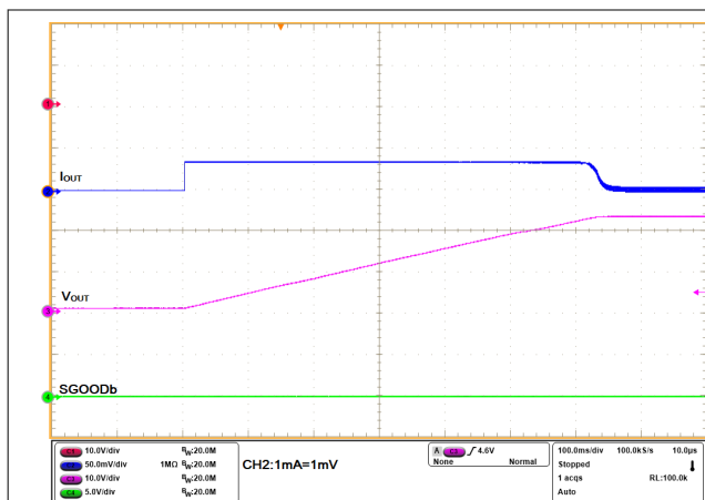
Figure 9-12. TPS26612: Startup of 2-Wire transmitter with MODE = GND, I_{OUT} = 30\text{ mA}
