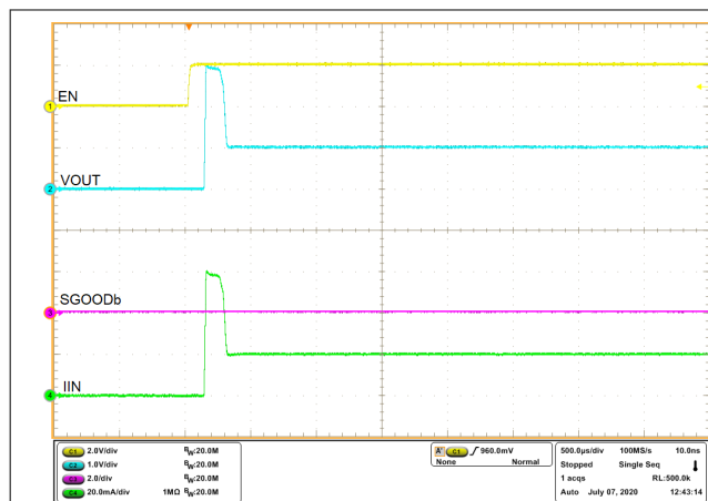
Figure 8-22. Turn-On With EN Pin
