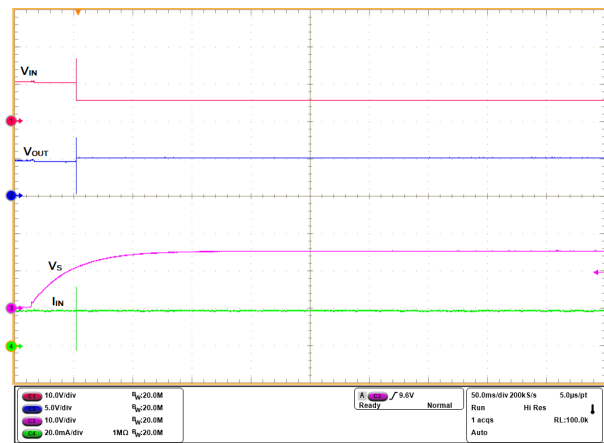
Figure 8-20. Transition to ± Vs Supplies Power with R1 = 47 kΩ and R2 = 6.8 kΩ for supply Sensing
