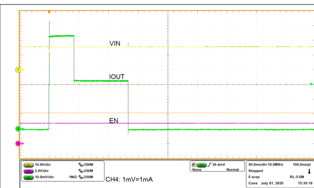
Figure 8-7. Current Limit Behavior for I_{OUT} > 2 \times I_{OL} with MODE = 180\text{ k}\Omega
