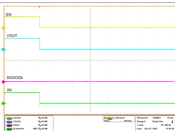
Figure 8-23. Turn-Off With EN Pin
