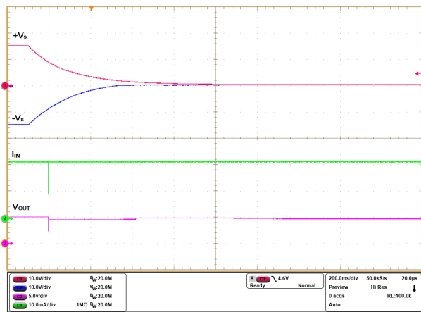
Figure 8-19. Transition to Loop Power With R1 = 47 kΩ and R2 = 6.8 kΩ for Supply Sensing
