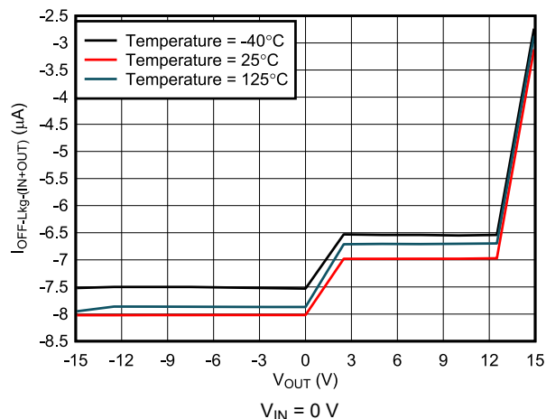
Figure 7-9. (I OFF-Leakage-IN + I OFF-Leakage-OUT ) vs V OUT
