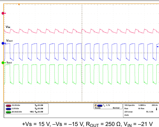
Figure 8-17. Thermal Protection During Loop Testing for I_{LOOP} < 0
