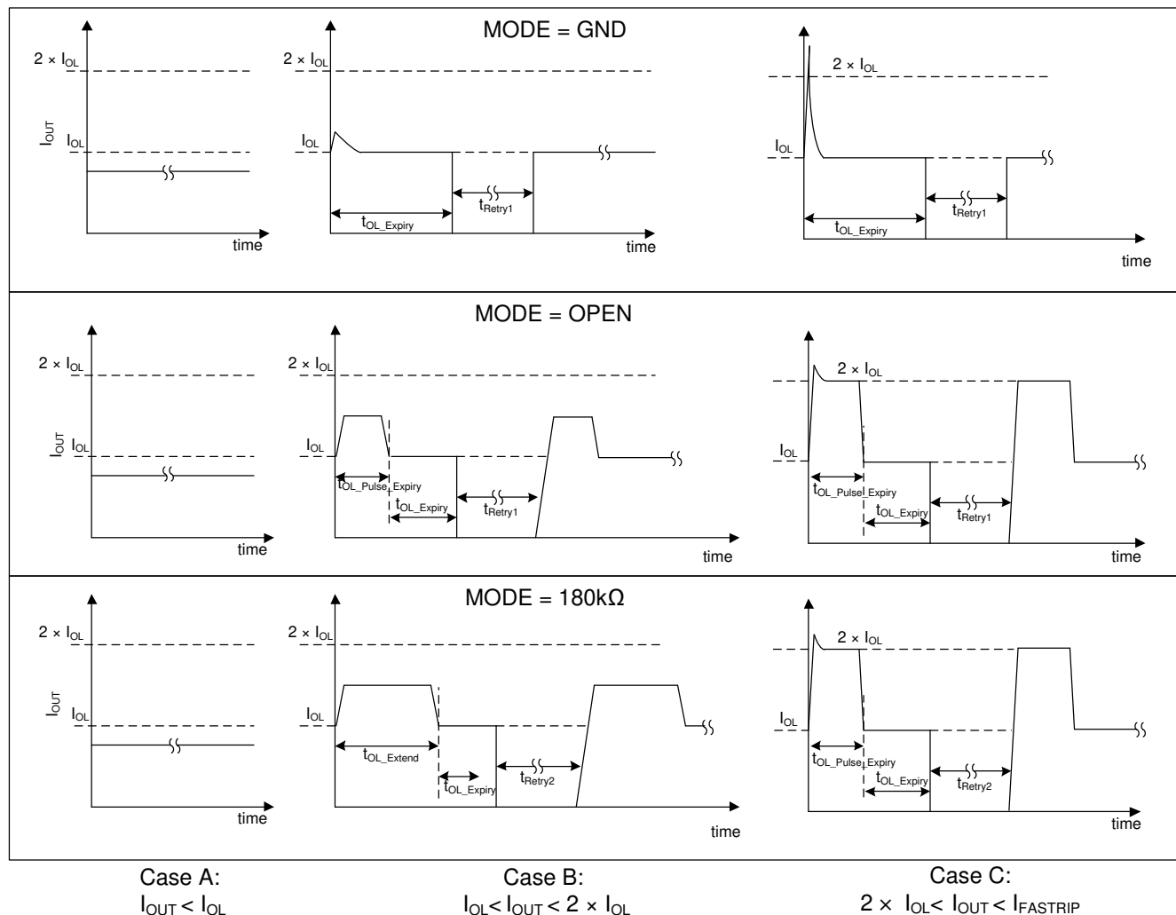
Figure 8-24. Device Operation Under Different MODE Configurations for I_{OL} > 0
