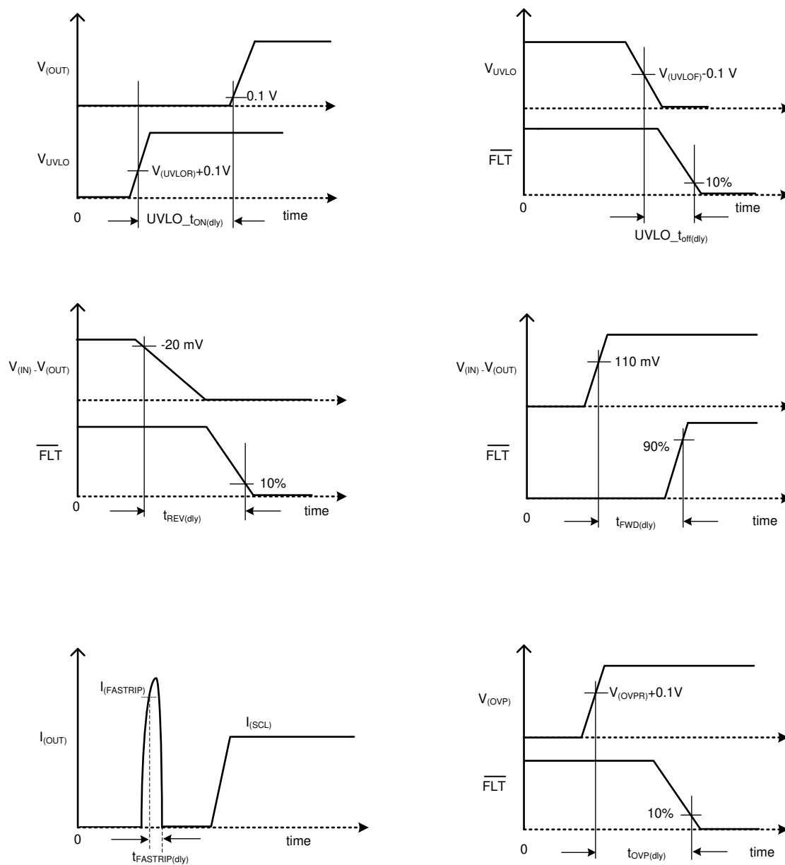
Figure 33. Timing Waveforms
