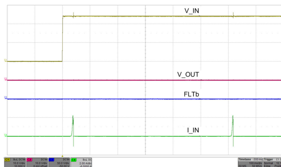
MODE pin connected to RTN VIN = 24 V R ILIM = 5.36 kΩ
