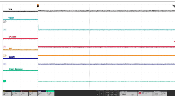
Figure 7-39. Power Cycle Using PMBus Command
