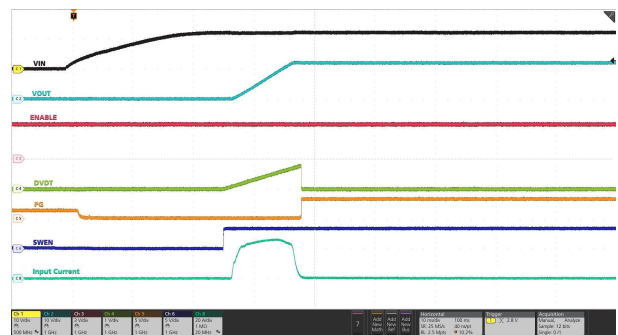
EN held high, IN supply ramped up to 12 V. C_{OUT} = 18 \text{ mF} , C_{dVdt} = 33 \text{ nF}
