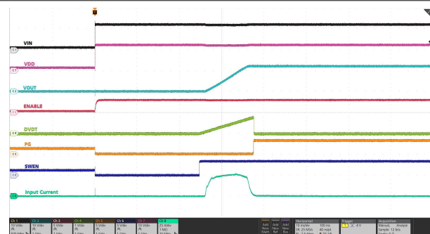
IN hot-plugged to 12 V supply. C_{OUT} = 18 \text{ mF} , C_{dVdt} = 33 \text{ nF} , Insertion Delay programmed to 25 ms (INS_DLY = 0x01)
