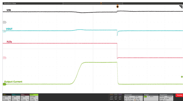
Figure 9-7. Power Up into Short: V_{IN} = 12 V, EN/UVLO Stepped Up From 0 V to 3 V, V_{IREF} = 1 V, R_{ILIM(TPS25990)} = 422 \Omega , R_{ILIM(TPS25985)} = 316 \Omega , and OUT Shorted to GND
