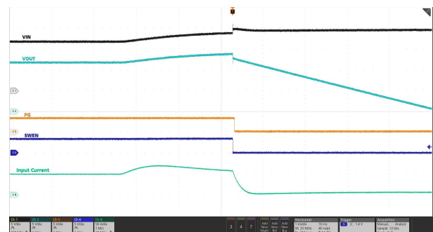
Figure 7-44. Input Undervoltage Protection
