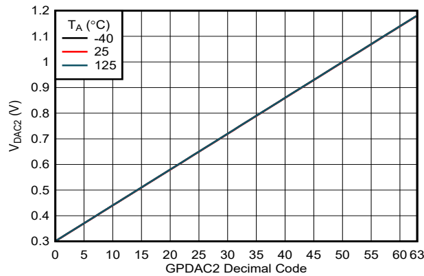
Figure 7-27. General Purpose DAC2 Transfer Function
