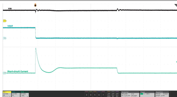
Figure 7-57. Short-Circuit Protection During Steady-state
