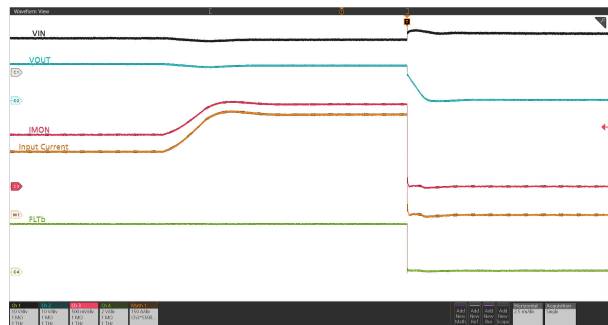
Figure 9-11. Circuit-Breaker Response: V_{IN} = 12\text{ V} , t_{OC\_TIMER} = 10\text{ ms} , C_{LOAD} = 50\text{ mF} , R_{IMON} = 150\ \Omega , V_{IREF} = 1\text{ V} , and Load Current Stepped from 333 A to 530 A for more than 10 ms
