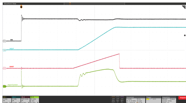
Figure 9-5. Input Hot Plug: V_{IN} Stepped Up from 0 V to 12 V, C_{LOAD} = 50 mF, R_{LOAD(Start-up)} = 0.48 \Omega , C_{DVRT} = 33 nF, V_{IREF} = 1 V, R_{ILIM(TPS25990)} = 422 \Omega , and R_{ILIM(TPS25985)} = 316 \Omega
