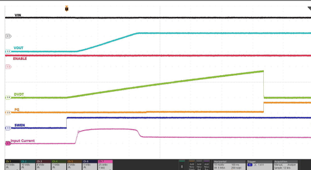
Figure 7-38. Power Up Using PMBus Command
