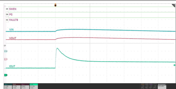
Figure 7-58. Short-Circuit Protection During Steady-state
