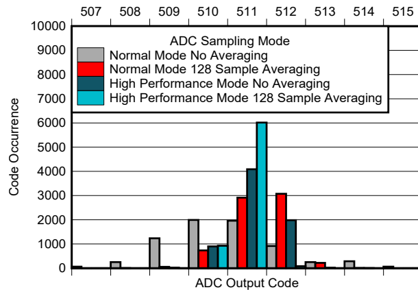
Figure 7-25. ADC Histogram (Mid-scale Analog Input)
