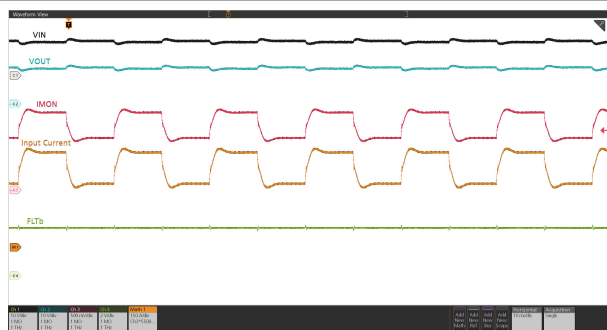
Figure 9-9. Transient Overload: V_{IN} = 12 V, t_{OC\_TIMER} = 10 ms, C_{LOAD} = 50 mF, R_{IMON} = 150 \Omega , V_{IREF} = 1 V, and Load Current Stepped from 333 A to 500 A then 333 A within 8.5 ms
