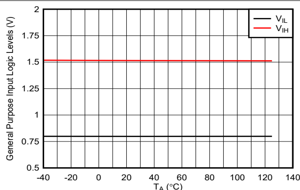
Figure 7-29. SWEN/General Purpose Input Pin Logic Thresholds Across Temperature
