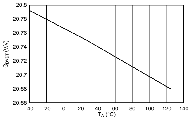
Figure 7-23. DVDT Gain Across Temperature
