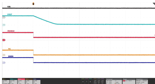
Figure 7-43. Power Down Using EN With Output Discharge
