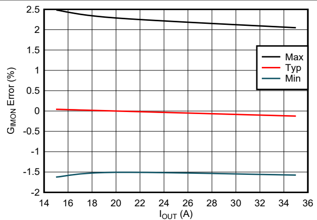
Figure 7-12. IMON Gain Accuracy Across Process, Voltage and Temperature Corners
