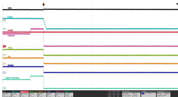
Figure 7-51. Transient Overcurrent Blanking
