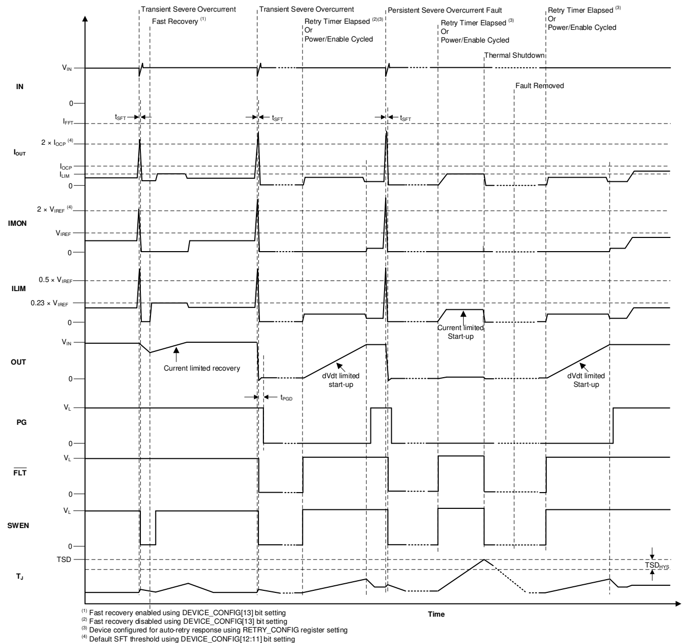
Figure 8-5. Short-Circuit Response
