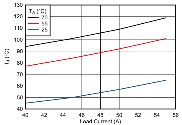
Figure 7-32. Junction Temperature vs Load Current (No Air-Flow)
