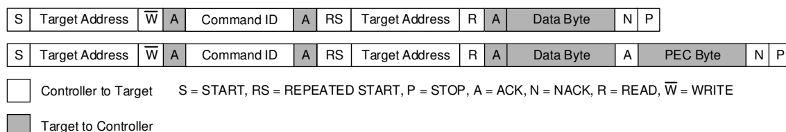
Figure 8-13. Read Byte
