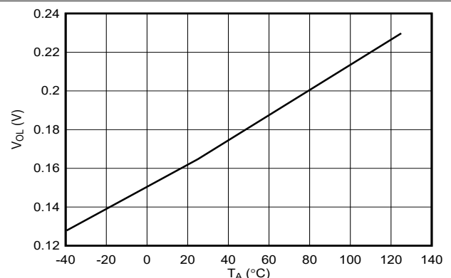
Figure 7-30. PGOOD/FLT/General Purpose Output Pin Logic Level Across Temperature
