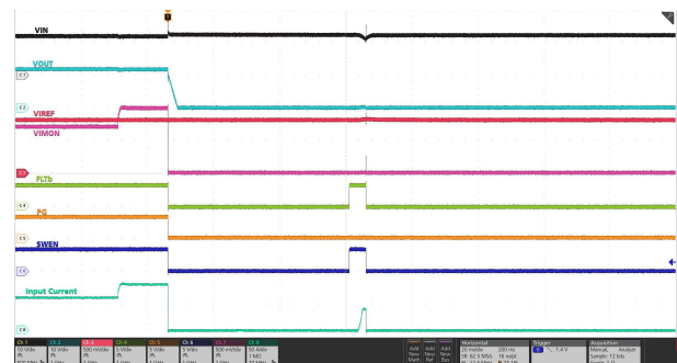
Figure 7-52. Overcurrent Protection
