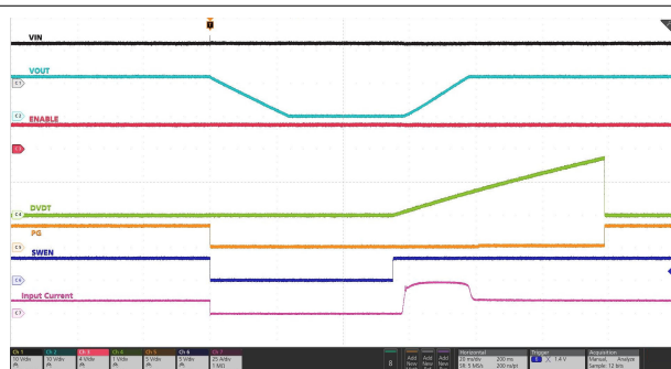
Figure 7-37. Power Down Using PMBus Command
