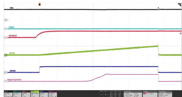
Figure 7-56. Power Up into Short-Circuit Protection
