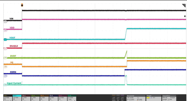
IN hot-plugged to 12 V supply. C_{OUT} = 18 \text{ mF} , C_{dVdt} = 33 \text{ nF} , Insertion Delay programmed to 560 ms (INS_DLY = 0x07)
