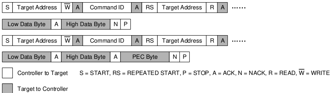
Figure 8-15. Read Word
