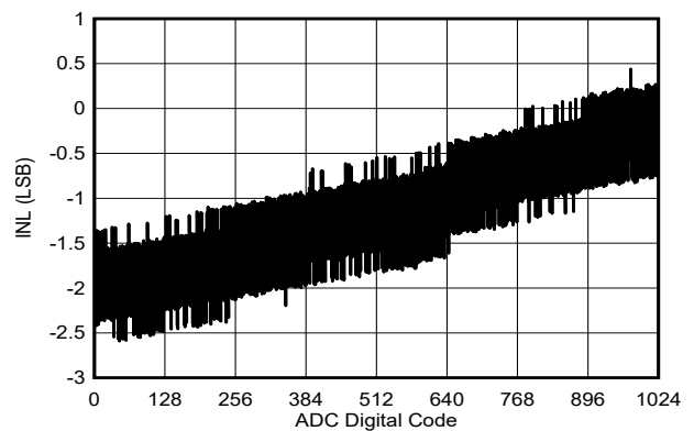
Figure 7-24. ADC INL
