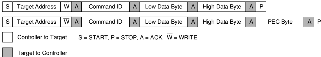
Figure 8-14. Write Word
