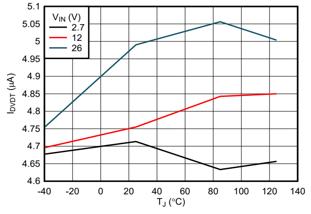
Figure 6-14. DVDVT Pin Charging Current vs Temperature
