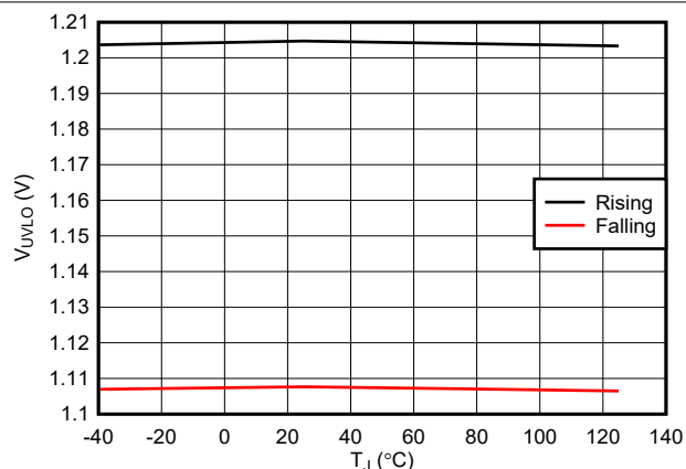
Figure 6-4. EN/UVLO Pin Threshold vs Temperature
