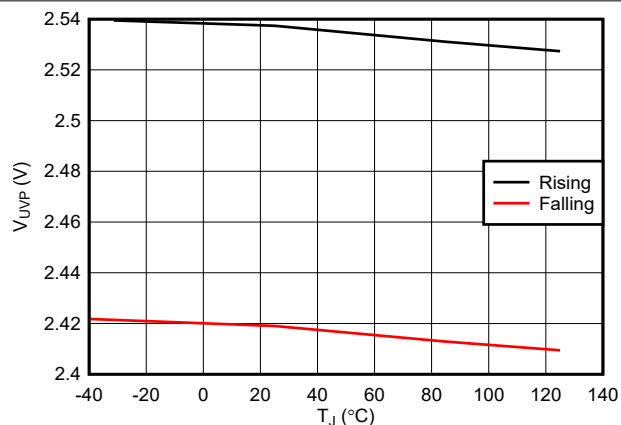
Figure 6-2. Supply UVP Threshold vs Temperature
