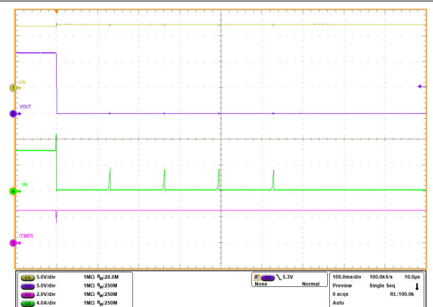
Figure 7-27. Overvoltage Protection
