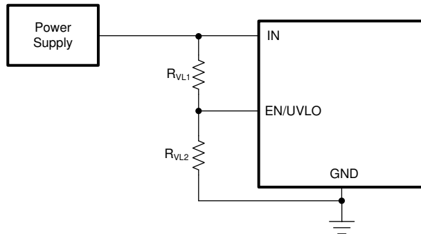
Figure 8-1. Adjustable Supply UVLO Threshold
