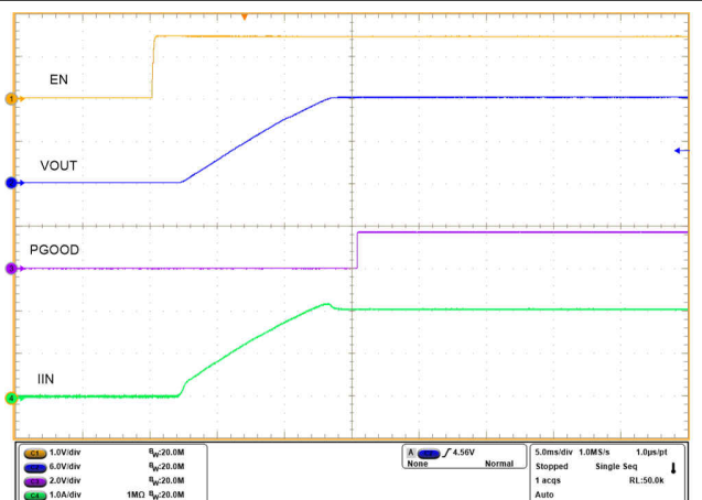
Figure 7-24. Hotplug
