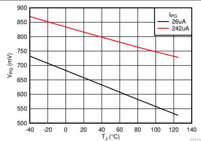
Figure 7-12. Power Good Output Voltage (De-asserted State) vs Temperature
