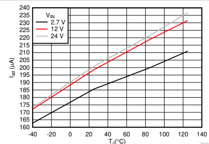
Figure 7-8. Shut-Down Current vs Temperature
