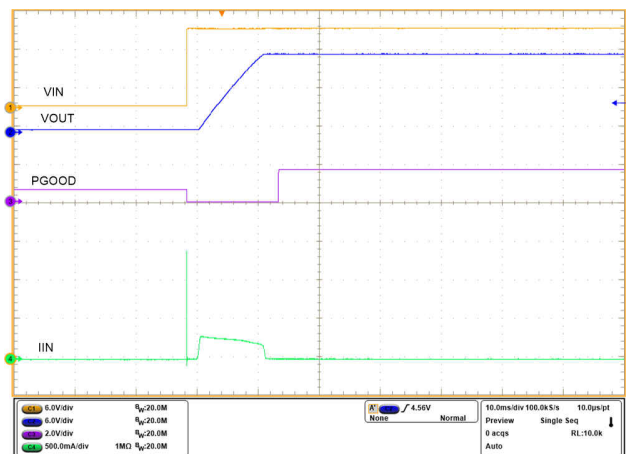
Figure 7-24. Hotplug
