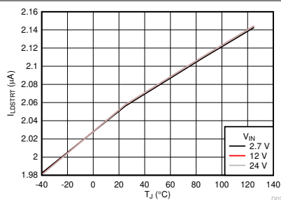
Figure 7-15. LDSTRT Charging Current vs Temperature
