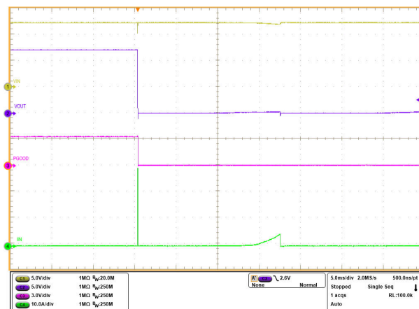
Figure 7-31. Output Hard Short-Circuit While ON
