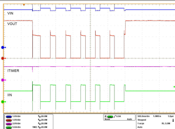
Figure 9-18. Overload Response and Recovery
